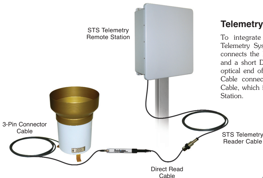
Tipping Bucket
